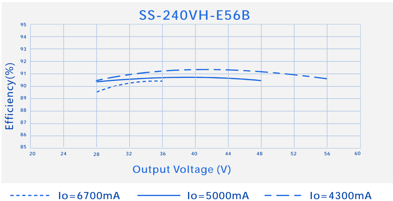
Efficiency Vs. O/P Voltage ( V_{in}=120Vac )
